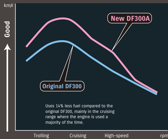
Comparison of Fuel Consumption per 1 Liter of Fuel (New DF300A vs. Original DF300)
